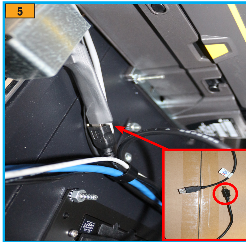
5.) Take the USB 3.0 cable included with the harness and plug it into the USB 3.0 port on the validator harness as shown.
