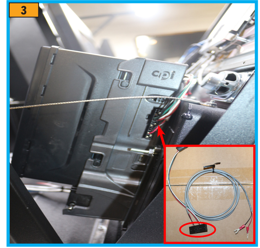
3.) Plug the crimp housing end of the new validator harness into the port you previously removed the old one from in the bill validator.
