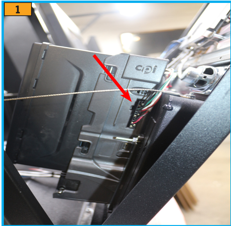
1.) Locate the crimp housing side of the existing kiosk validator harness that's plugged into the validator. Unplug this connection.
