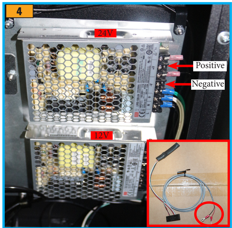
4.) Identify the positive and the negative sides of the bill validator harness respectively. Connect the positive and negative ends into the proper location using the screws you previously removed with the Phillips head.
